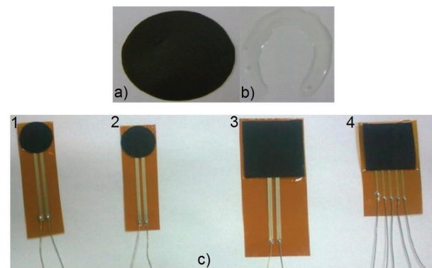
Figure 2: a) Printed carbon ink, b) mounted two component epoxy glue and c) four types of FSR sensors after manufacturing, respectively
